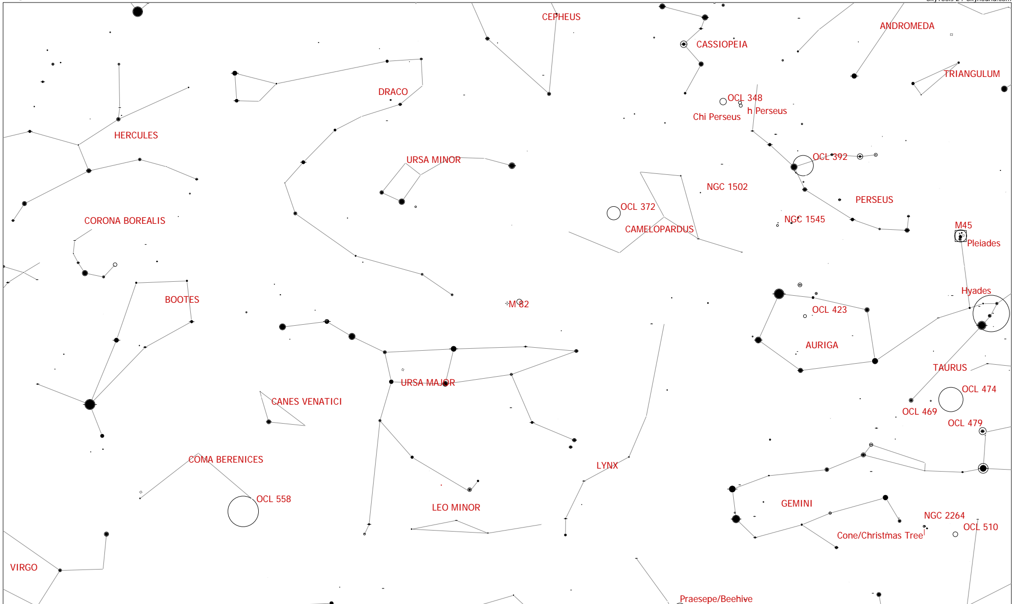
M 82 (Galaxy) aka NGC 3034, Arp 337, PGC 28655, MCG 12-10-11, UGC 5322 RA: 09h55m52.2s Dec: +69°40'49" J2000 (UMa) Mag: 9.20 Size: 10.5'x 4.4' Irregular, Nearly edge on SBr: 22.0 Mag/arc-sec 2
