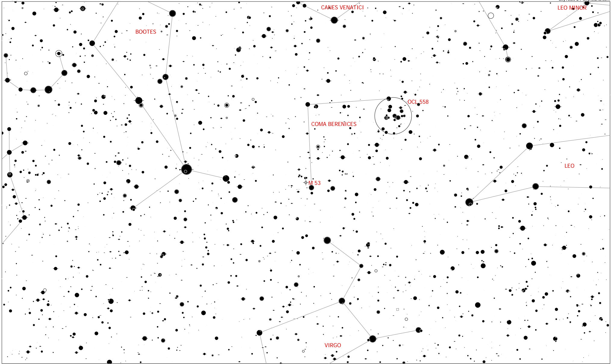
M 53 (Globular Cluster) aka NGC 5024 RA: 13h12m55.0s Dec: +18°10'12" J2000 (Com) Mag: 7.70 Size: 13.0' Distance: 65000 ly
